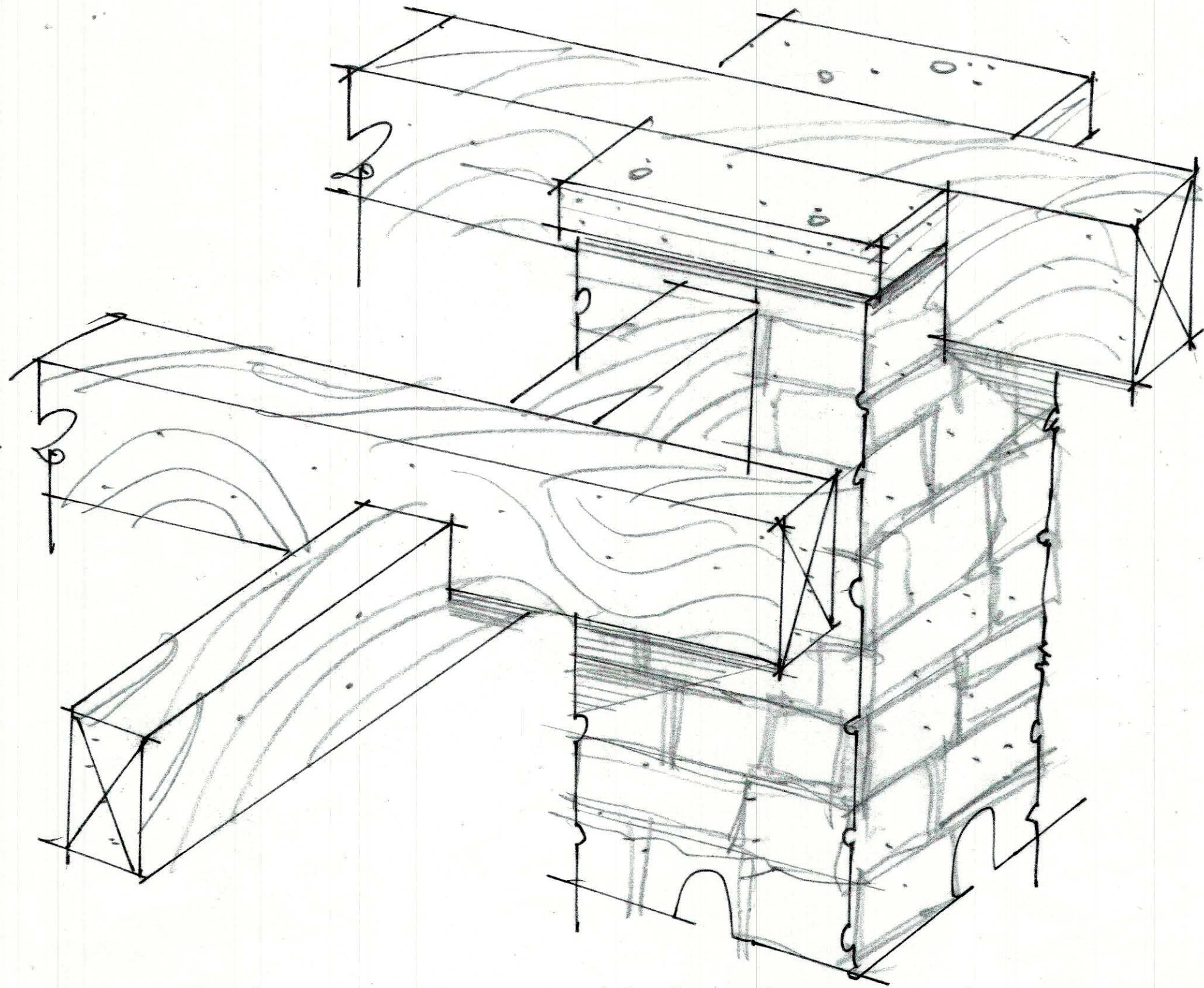
Column - Beam - Joist Connection N.T.S. / Isometric
